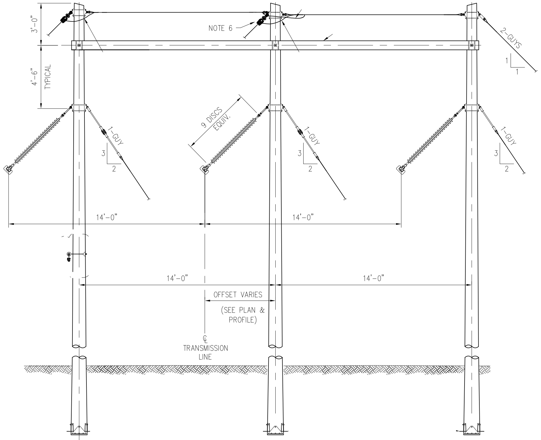
3 POLE GUYED ANGLE
