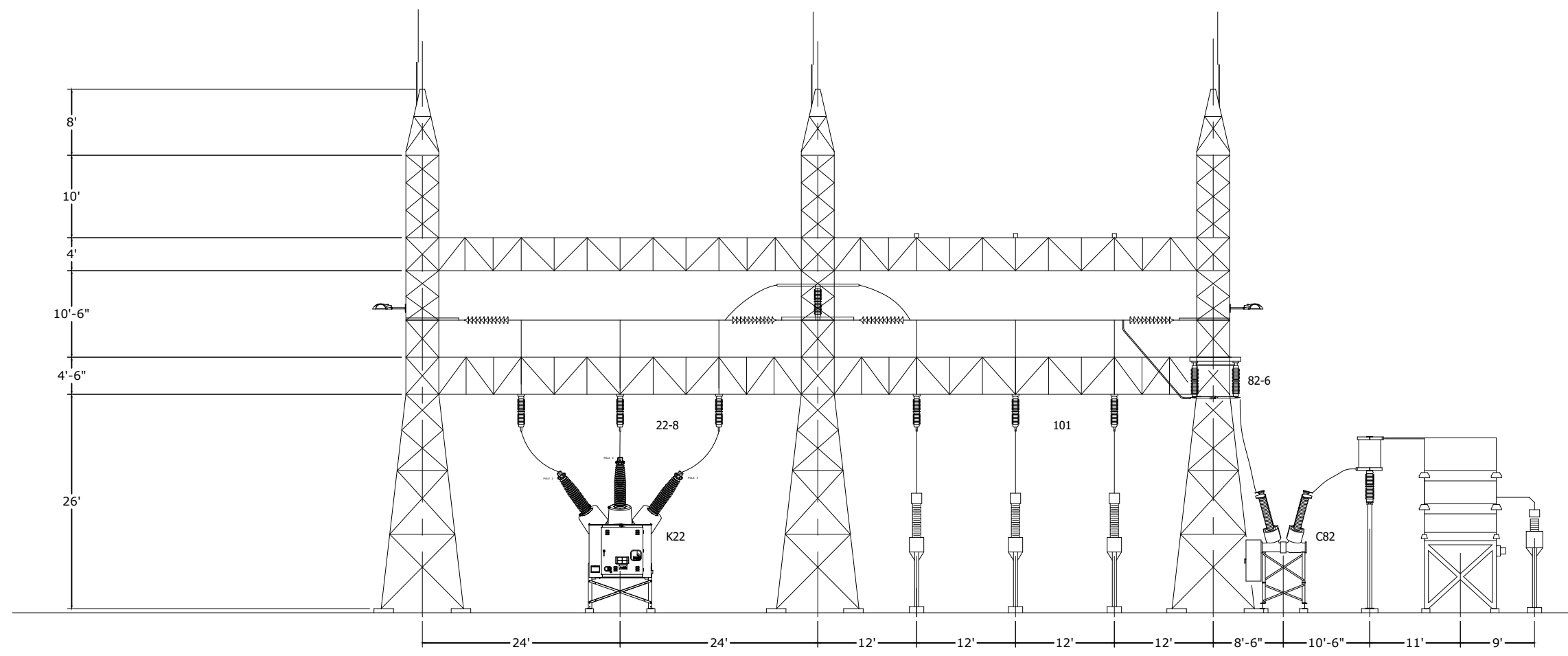
SECTION B-B
